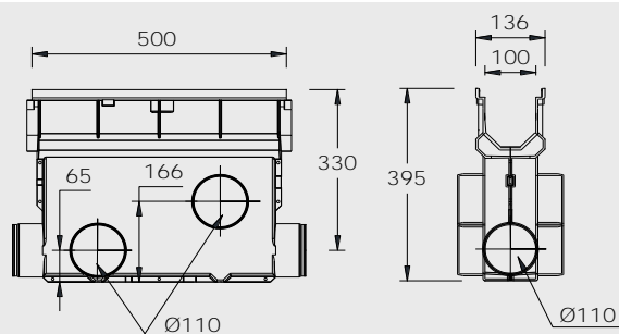
MEAFLUID 100 EK
